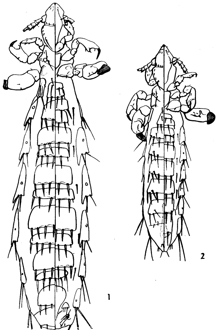
Polyplox meridionalis , new species. Fig. 1, female allotype; fig. 2, male holotype.
