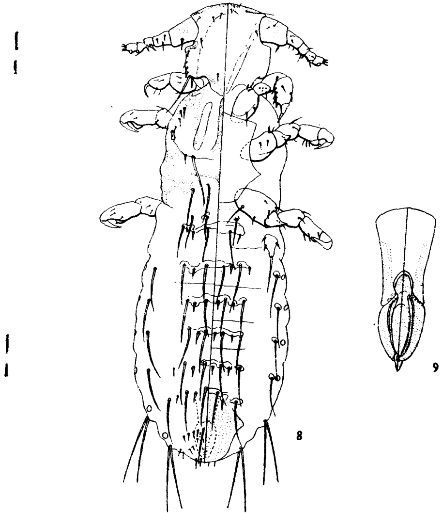
Lemurphthirus stigmatosus Ferris. Fig. 8, male from Galago senegalensis , Angola; fig. 9, genitalia, male.
