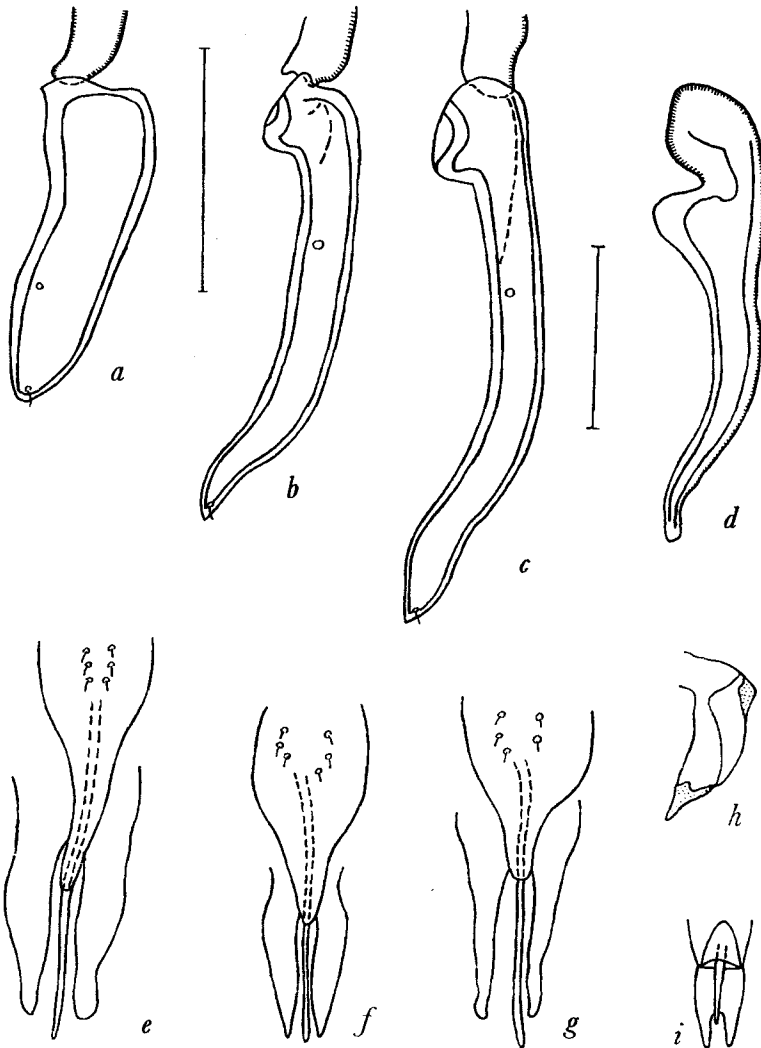
FIGURE 1.— a , Saemundsonia parvigenitalis , paramere (holotype); b , S. petersi , paramere (holotype); c , S. snyderi , paramere (lectotype); d , S. petersi , endomere (holotype); e , S. meridiana , mesosome (holotype); f , S. petersi , mesosome (holotype); g , S. snyderi , mesosome (lectotype); h , S. parvigenitalis , endomere (holotype); i , S. parvigenitalis , mesosome (holotype). The vertical line to the right of figure c represents 0.10 mm. Figure b is drawn to the same scale. The scale of the remaining figures is represented by the line to the right of figure a and is also equivalent to 0.10 mm.
