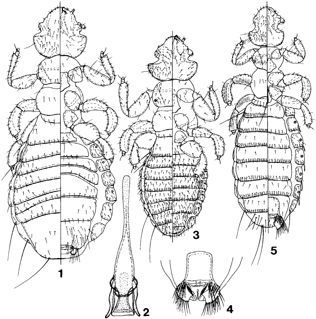
Figs. 1-5. 1-3, Glicicola cutkompi . 1, Female, dorsoventral. 2, Male genitalia. 3, Male, dorsoventral. 4-5, G. brooksae . 4, Female ventral terminalia. 5, Female, dorsoventral.
