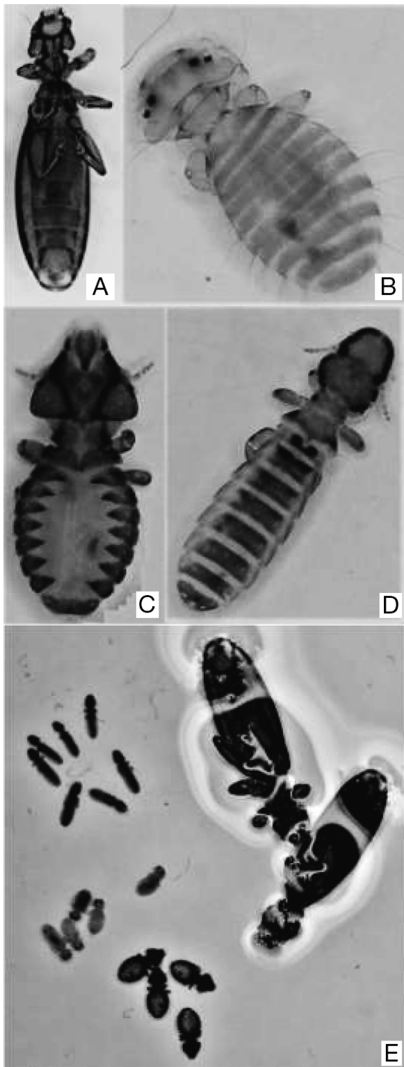
Figure 1. Specimens of buzzard lice in alcohol (70%) under stereo microscope (A) Laemobothrion maximum , (B) Colpocephalum nanum , (C) Craspedorrhynchus platystomus , (D)
